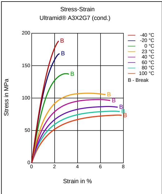
Stress-strain
